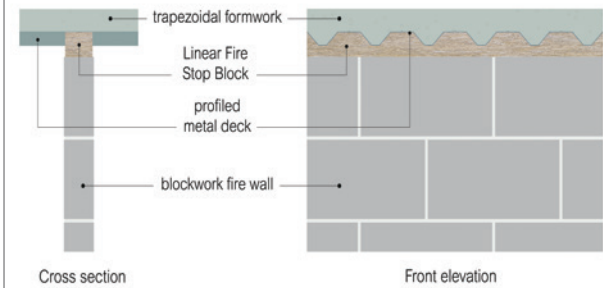
Linear Fire Stop Block at the head of a masonry wall
