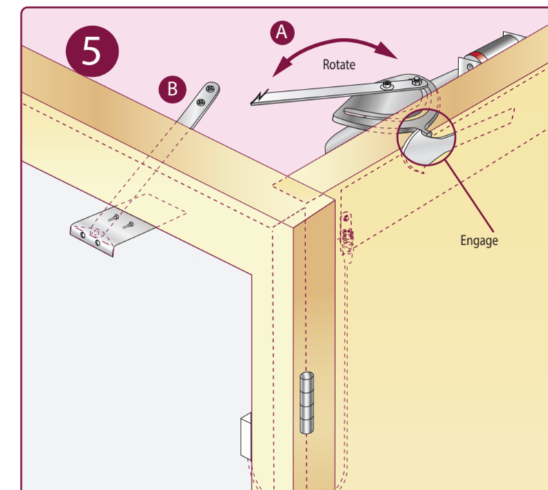
A. Open door and rotate pinion through 90° with arm and engage Arc wheel with Hold Open catch plate. B. Separate the arm assembly and connect to the soffit bracket. Longest side of the shoe towards the hinge. C. Fasten secondary arm together, switch off electricity so the closer shuts the door. D. Adjust secondary arm so it holds parallel to the frame and tighten the two lock nuts.
